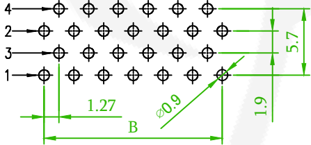
Recommended P.C.B Layout (Top Side) (PCB BOAED TOLERANCE±0.05)
