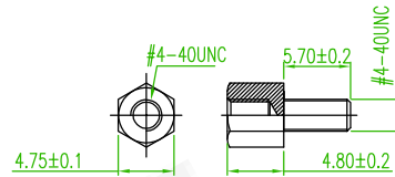
B: Thread Insert #4-40 + Jack Screw #4-40 Attached
