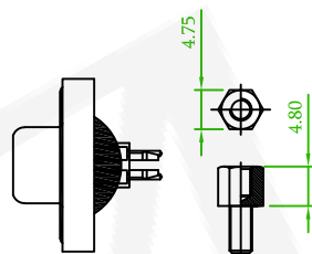
57WDDXSXM-XXBBXXBA-01 Thread Insert #4-40 + Jack Screw #4-40 Attached
