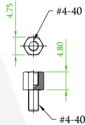
57WDD SXF-XXBBXXBA-01 Thread Insert #4-40 + Jack Screw #4-40 Attached
