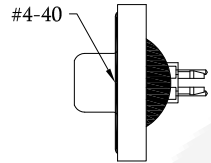
57WDD SXF-XXBAXXBA-01 Thread Insert #4-40
