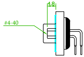
57WDDRXF-XXXCXXA-03 Thread Insert #4-40 UNC + Jack Screw #4-40 UNC Removable
