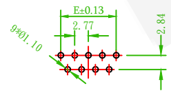
Recommended PCB Layout (PCB TOLERANCE ±0.05)
