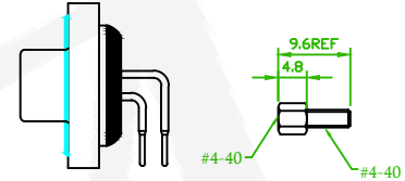
57WDDRXF-XXXBXXA-03 Thread Insert #4-40 + Jack Screw #4-40 Attached
