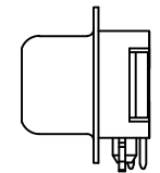
Thread Insert #4-40 + Jack Screw #4-40 Attached
