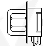
Thread Insert #4-40 + Jack Screw #4-40 Removable
