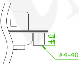
57PDSS4M-C4NFN1BAJ-X1 Rear Rivet Thread Insert #4-40 UNC H4.0
