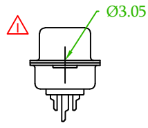
N: Clear Hole \varnothing 3.05mm 57HDSSXM-XXNNXXA-01
