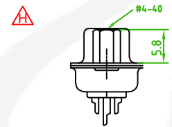
Front Rivet #4-40, H=5.8 57HDSSXM-XXNHXXA-01
