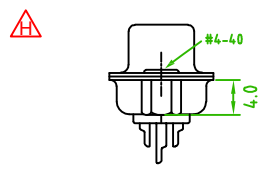
Rear Rivet #4-40, H=4.0 57HDSSXM-XXNFXXA-01
