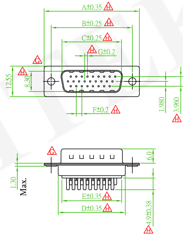
N: Clear Hole \varnothing 3.05mm 57HDSSXM-XXNNXXA-01
