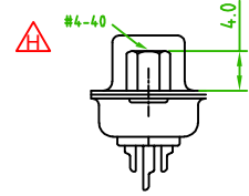
Front Rivet #4-40, H=4.0 57HDSSXM-XXNDXXA-01
