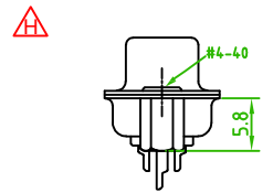
Rear Rivet #4-40, H=5.8 57HDSSXM-XXNIXXA-01
