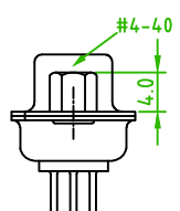
Front Rivet #4-40 H:4.0 57HDDSXF-XXNDXXA-01
