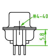
Rear Rivet #4-40 H:5.8 57HDDSXF-XXNIXXXA-01
