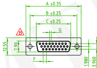
Front Rivet #4-40 H:4.0 57HDDSXF-XXNDXXA-01
