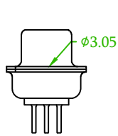
#3.05 Clear Hole W/O Boardlock 57HDDSXF-XXNXXXXA-01
