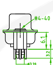
Thread Insert #4-40+ Jack Screw #4-40 Attached With Boardlock 57HDDSXF-XXBBXXA-01
