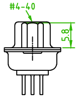
Front Rivet #4-40 H:5.8 57HDDSXF-XXNHXXA-01
