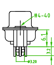
Thread Insert #4-40 UNC With Boardlock 57HDDSXF-XXBAXXXA-01
