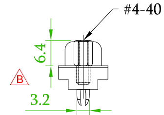
57DBDSXM-XXCCXXXXA-A1 With Boardlock Thread Insert #4-40 +Jack Screw #4-40 Removable
