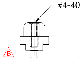
57DBDSXM-XXNCXXXXA-A1 Thread Insert #4-40 +Jack Screw #4-40 Removable
