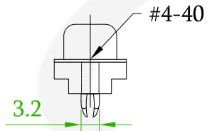
57DBDSXM-XXBAXXXA-A1 With Boardlock Thread Insert #4-40
