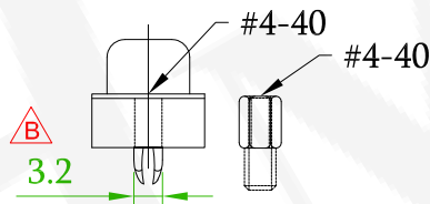
57DBDSXM-XXBBXXXXA-A1 With Boardlock Thread Insert #4-40 +Jack Screw #4-40 Attached
