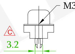
57DBDSXM-XXBOXXXA-A1 With Boardlock Thread Insert M3
