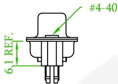
With Boardlock +Thread Insert #4-40 57DBDSXF-XXBAXXXXXA-XX
