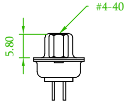
Front Rivet #4-40, H:5.8 57DBDSXF-XXNHXXXXA-XX
