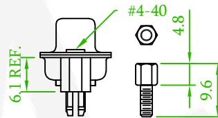
With Boardlock +Thread Insert #4-40 + Jack Screw #4-40 Attached ⚠ 57DBDSXF-XXBBXXXXA-XX
