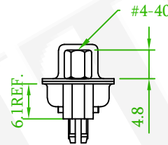
With Boardlock +Thread Insert #4-40 +Jack Screw #4-40 Removable 57DBDSXF-XXCCXXXXA-XX
