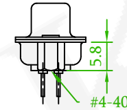
⚠ Rear Rivet #4-40, H:5.8 57DBDSXF-XXNIXXXXXA-XX
