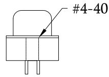
W/O Boardlock Thread Insert #4-40 57DBDSXF-XXNAXXXA-A1
