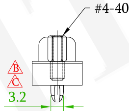
With Boardlock Thread Insert #4-40 +Jack Screw #4-40 Removable 57DBDSXF-XXBCXXA-A1
