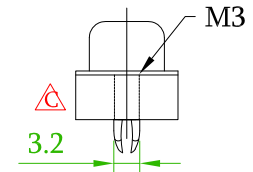
With Boardlock Thread Insert M3 57DBDSXF-XXBUXXXA-A1
