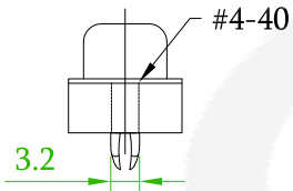
With Boardlock Thread Insert #4-40 57DBDSXF-XXBAXXXA-A1
