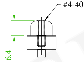
W/O Boardlock Thread Insert #4-40 +Jack Screw #4-40 Removable 57DBDSXF-XXNCXXXXA-A1
