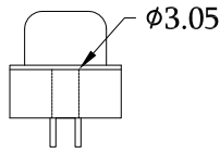
W/O Boardlock Ø3.05 Clear Hole 57DBDSXF-XXNNXXXXA-A1
