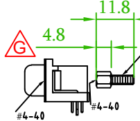
57DBDRXA-XXABXXBA-01 Thread Insert #4-40 + Jack Screw #4-40 Attached
