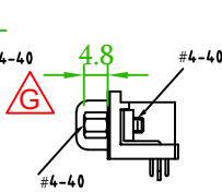
57DBDRXA-XXACXXBA-01 Thread Insert #4-40 + Jack Screw #4-40 Removable + Rivet ground strap
