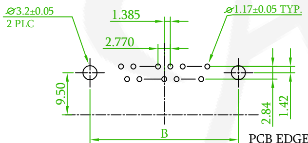
57DBDRXA-XXAHXXBA-01 Front Rivet #4-40 H=5.8
