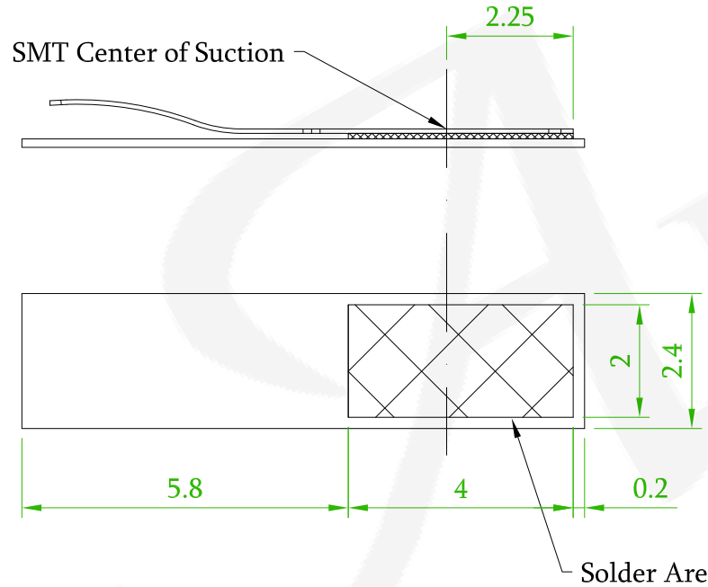
Recommended PCB Layout (PCB TOLERANCE \pm 0.1 )
