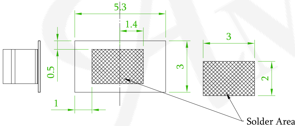
Recommended PCB Layout (PCB TOLERANCE \pm 0.1 )
