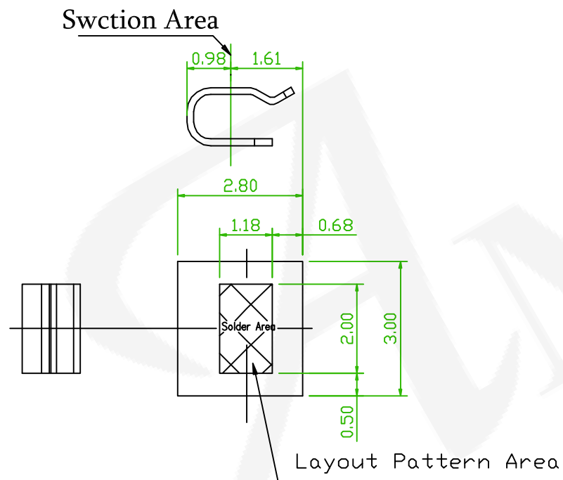
PCB Recommend Layout Pattern
