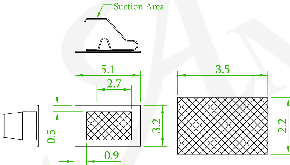
Recommended PCB Layout (PCB TOLERANCE ±0.1)
