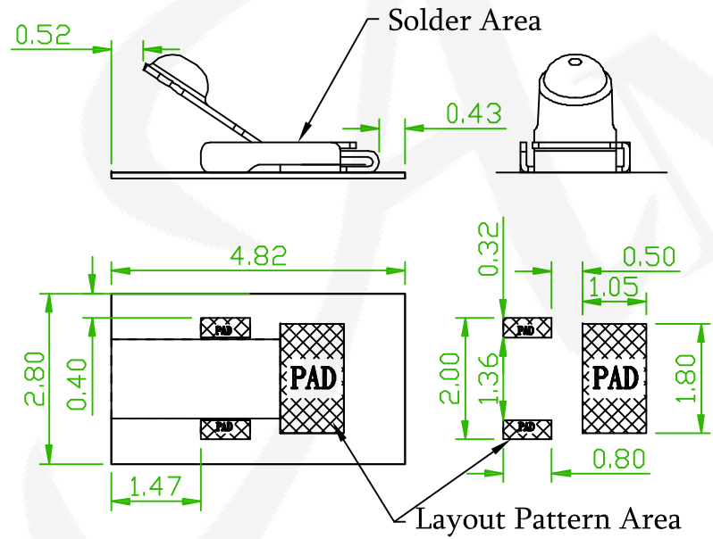
Recommended PCB Layout (PCB TOLERANCE ±0.1)
