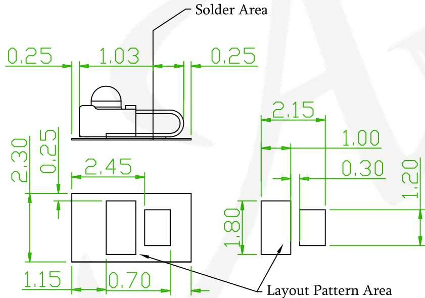
Recommended PCB Layout (PCB TOLERANCE ±0.1)
