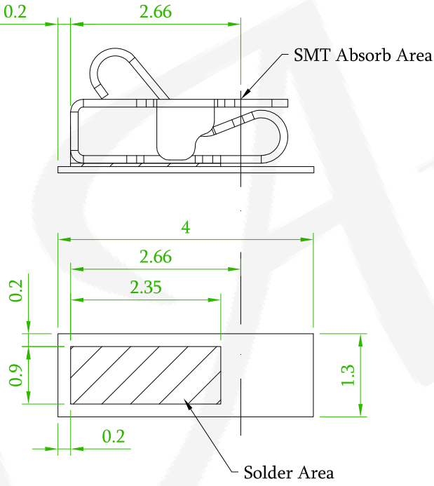
Recommended PCB Layout (PCB TOLERANCE ±0.1)
