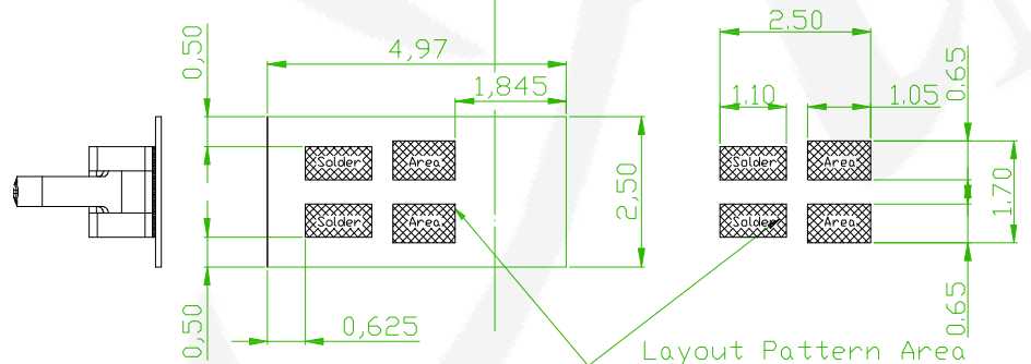
Recommended PCB Layout (PCB TOLERANCE \pm 0.1 )
