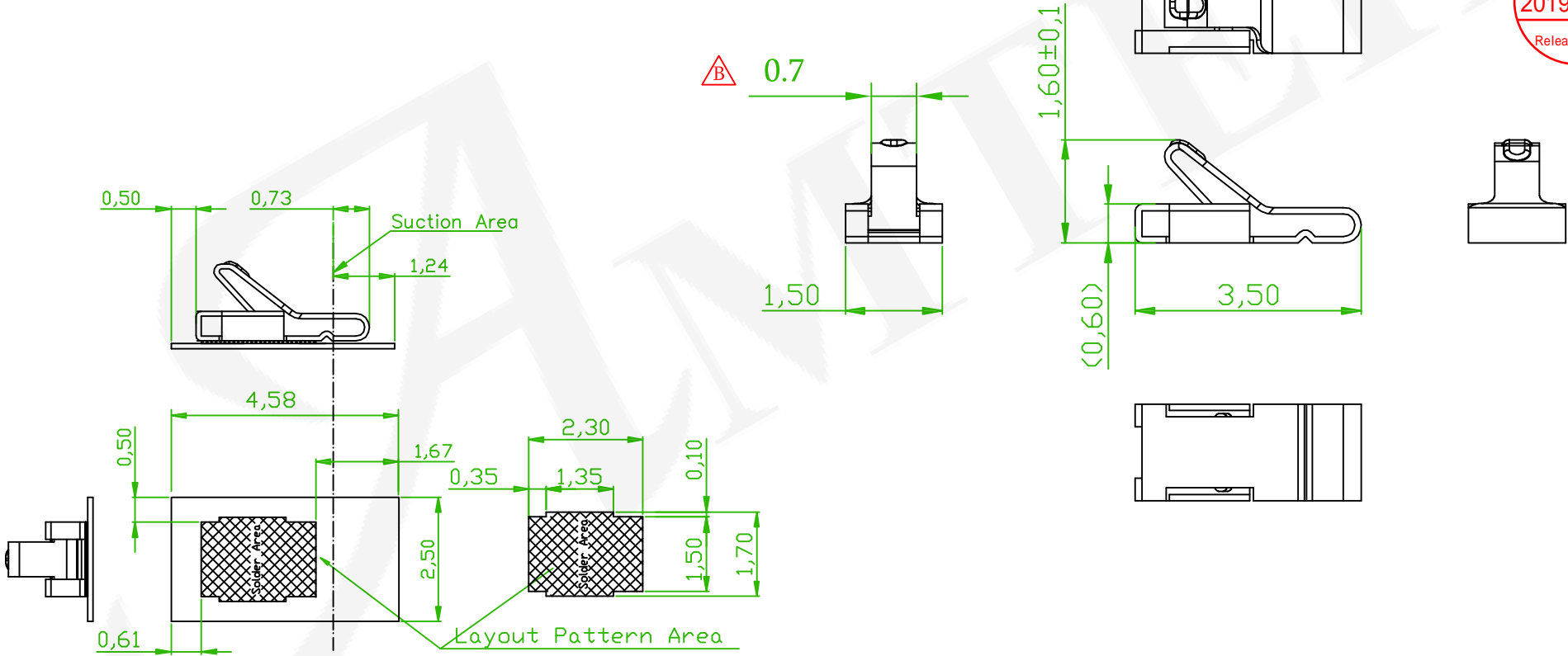
Recommended PCB Layout (PCB TOLERANCE \pm 0.1 )
