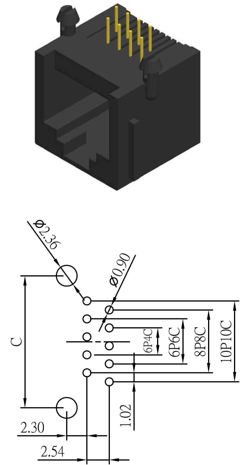
Recommended PCB Layout (PCB TOLERANCE ±0.05)
