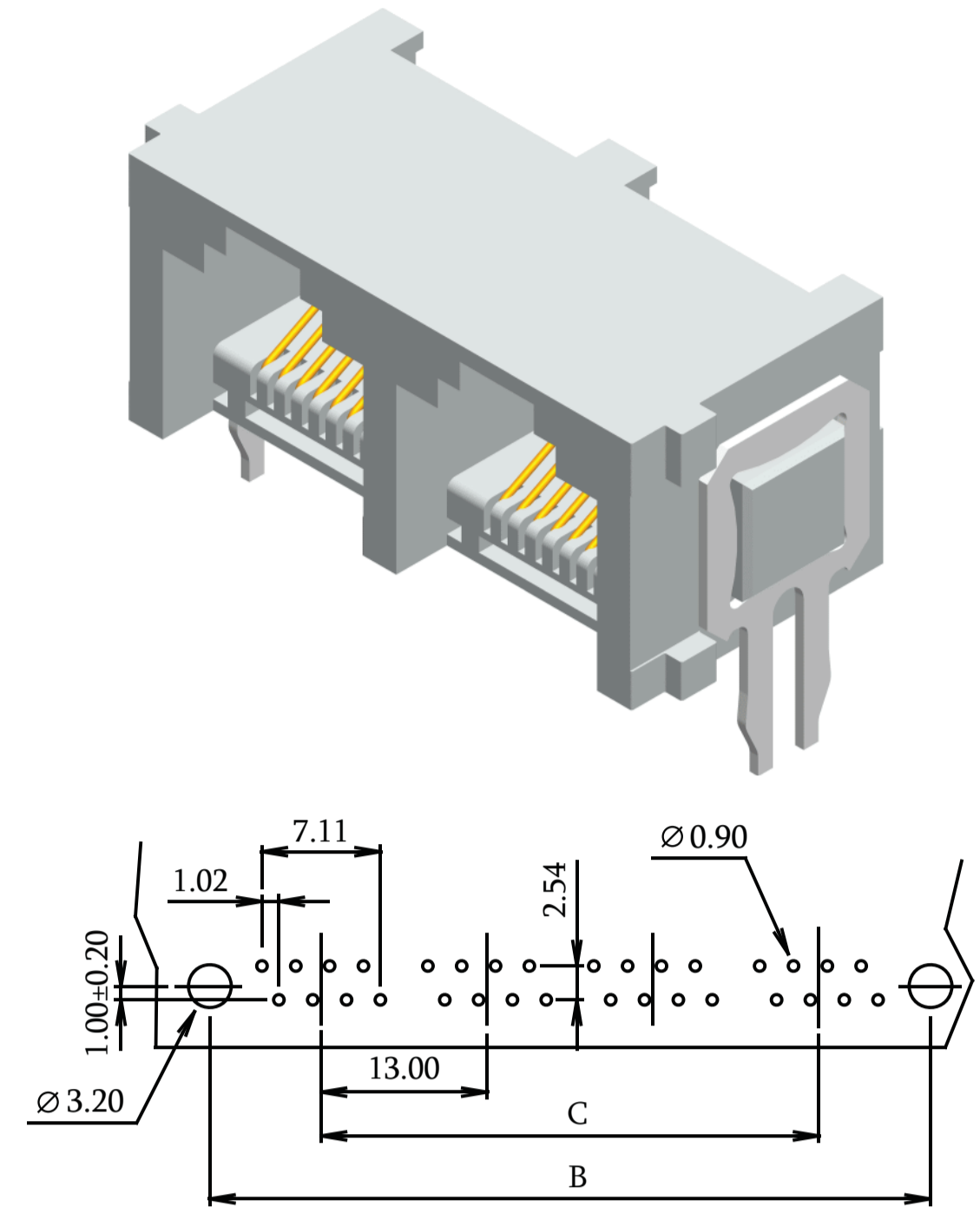
PC Board Layout
