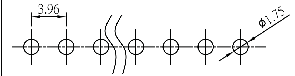
Recommended PCB Layout (PCB TOLERANCE \pm 0.05 )
