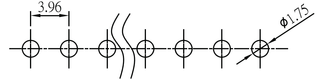
Recommended PCB Layout (PCB TOLERANCE \pm 0.05 )
