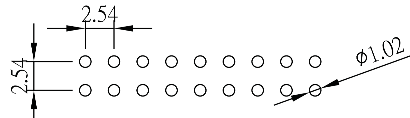
Recommended PCB Layout (PCB TOLERANCE ±0.05)
